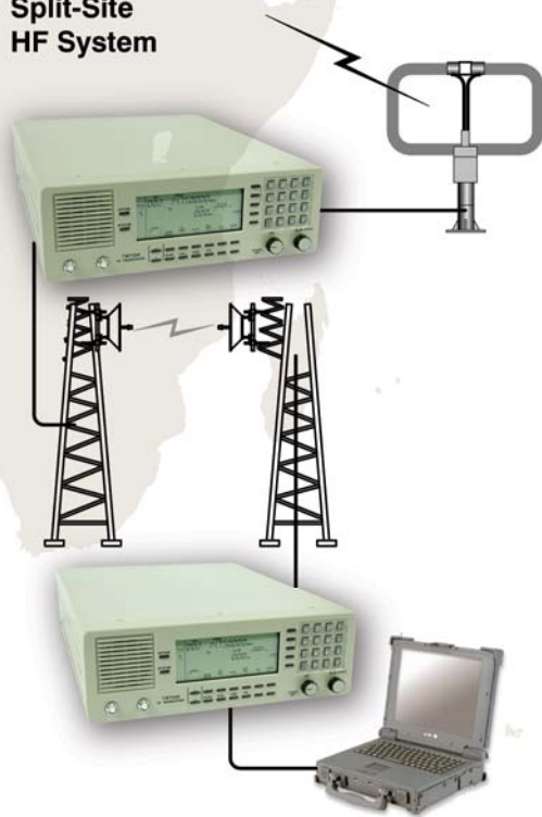
HF Ground-to-Air System using SELCAL
