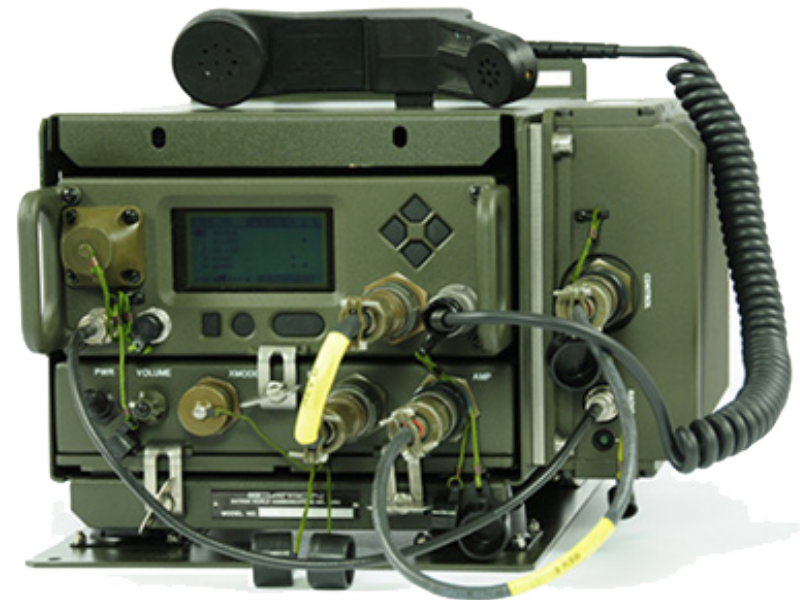
PRC2100V Manpack Radio, MT2100 Mobile Adapter, AM2100 Amplifier mounted in the MT2100-MM Mobile Mount
