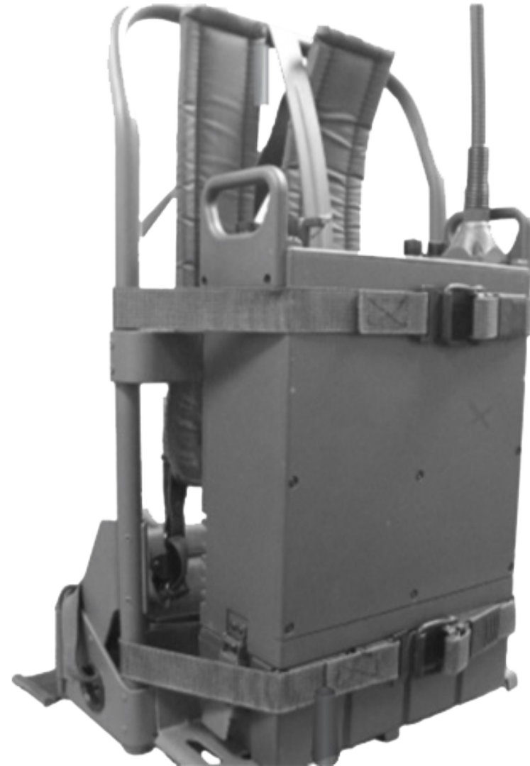
PRC7700H Transceiver with LC-2VS Backpack Frame
