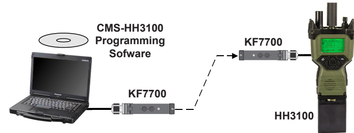
HH3100-DATA-CBL Data Cable
